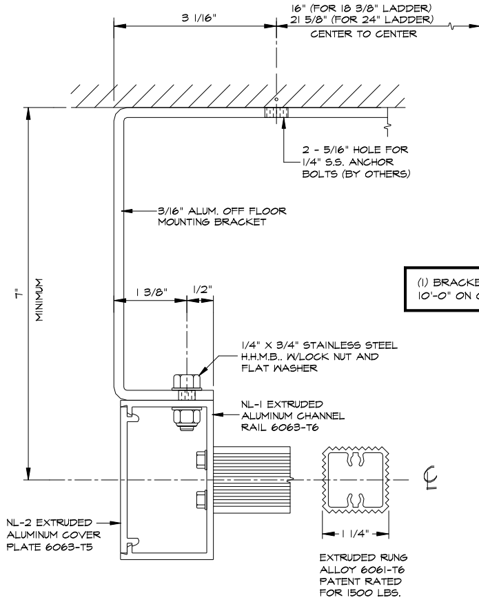
WALL BRACKET 1/2 FULL SCALE
