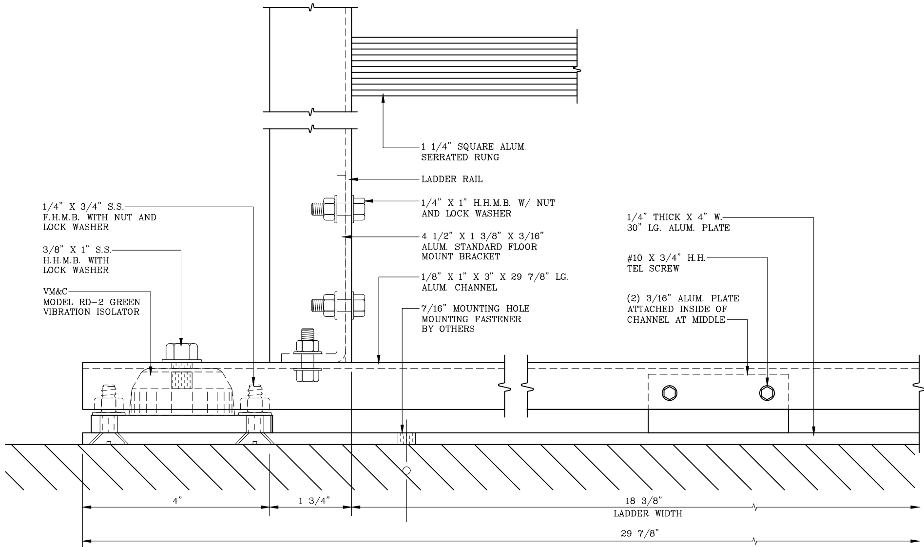
SEISMIC MOUNTING BRACKET FRONT VIEW (OPTIONAL) 1/2 FULL SCALE
