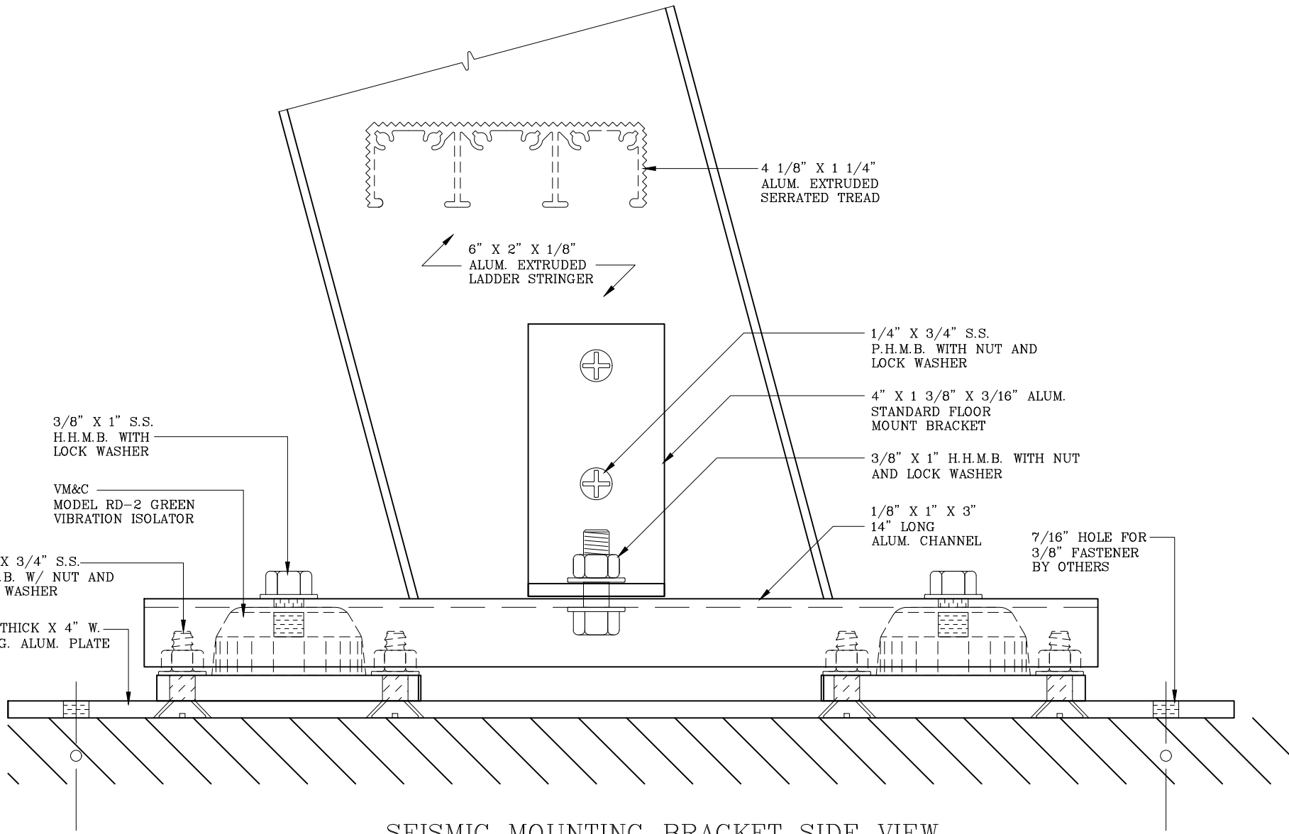
SEISMIC MOUNTING BRACKET SIDE VIEW (OPTIONAL) 1/2 FULL SCALE
