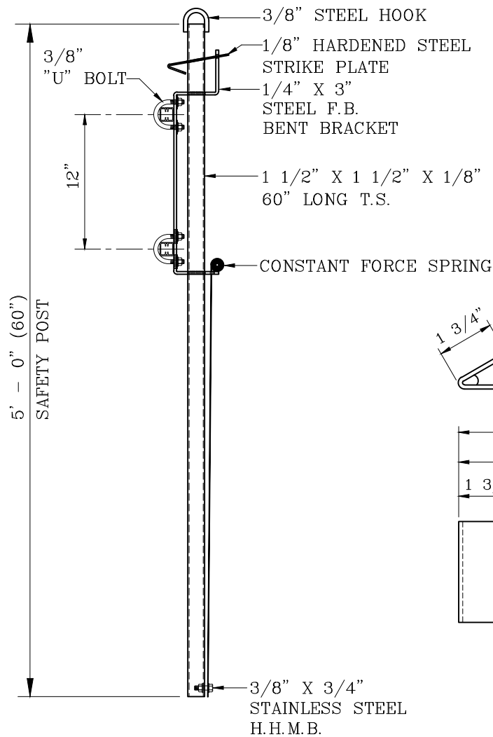
SAFETY POST 1" = 1' - 0"
