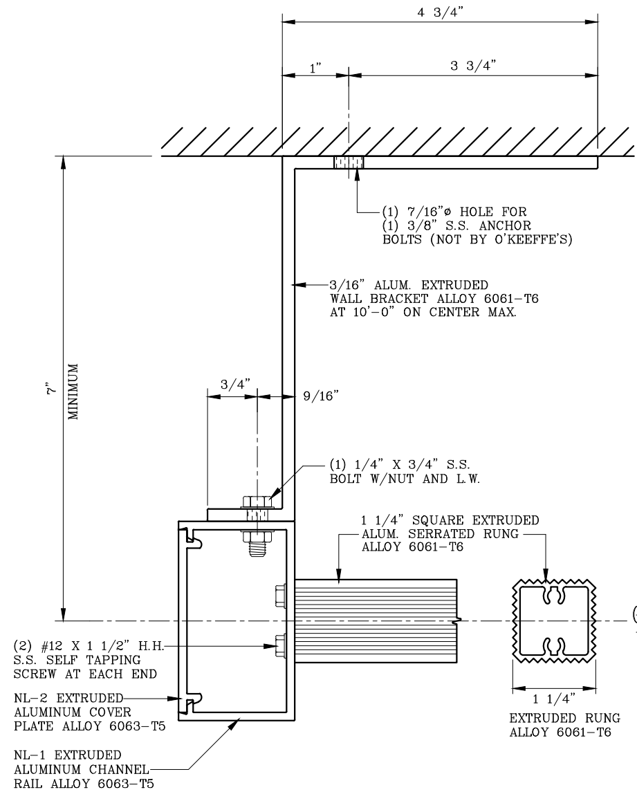
2 INTERMEDIATE BRACKET TOP VIEW 1 1/2 FULL SCALE
