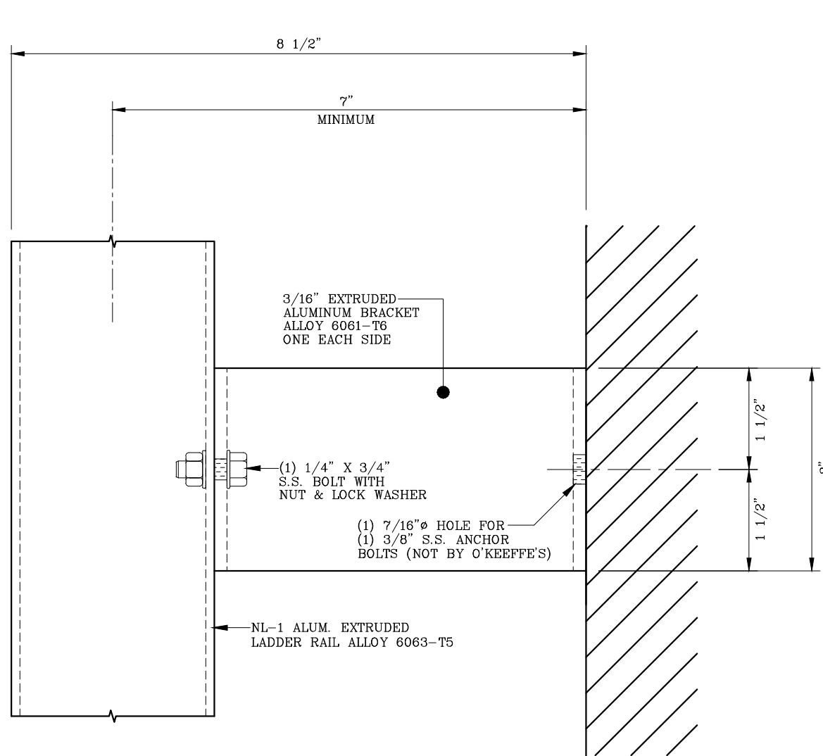
1 INTERMEDIATE BRACKET SIDE VIEW 1 1/2 FULL SCALE
