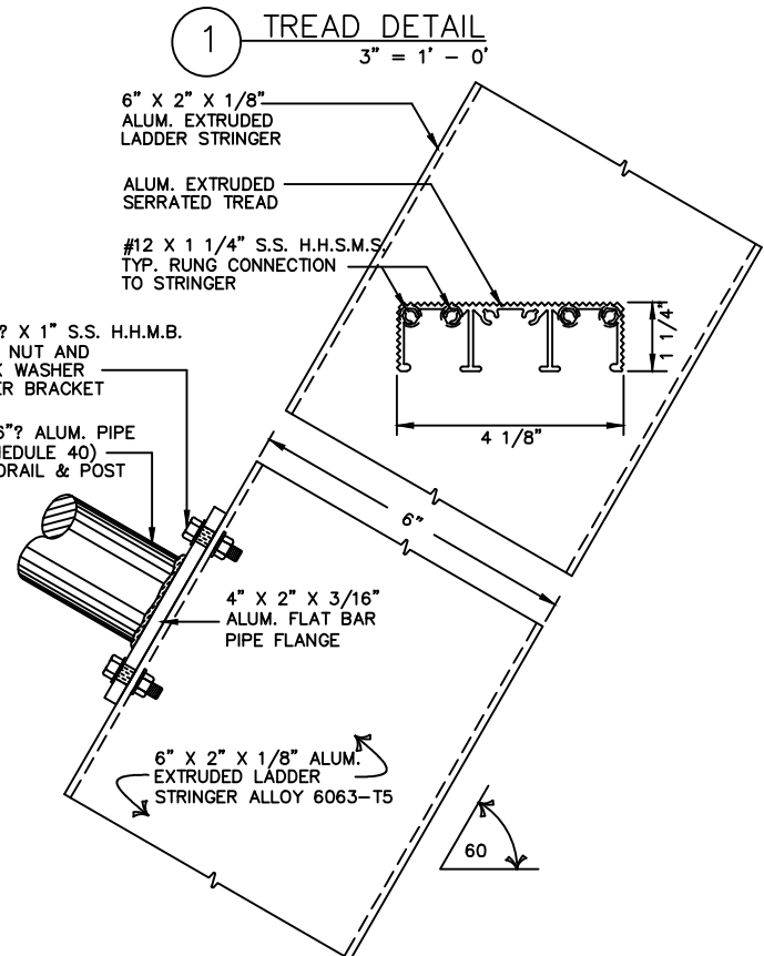
(2) POST DETAIL 3" = 1' - 0"
