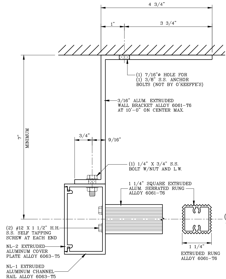
2 1 ADDITIONAL INTERMEDIATE BRACKET TOP VIEW 1/2 FULL SCALE
